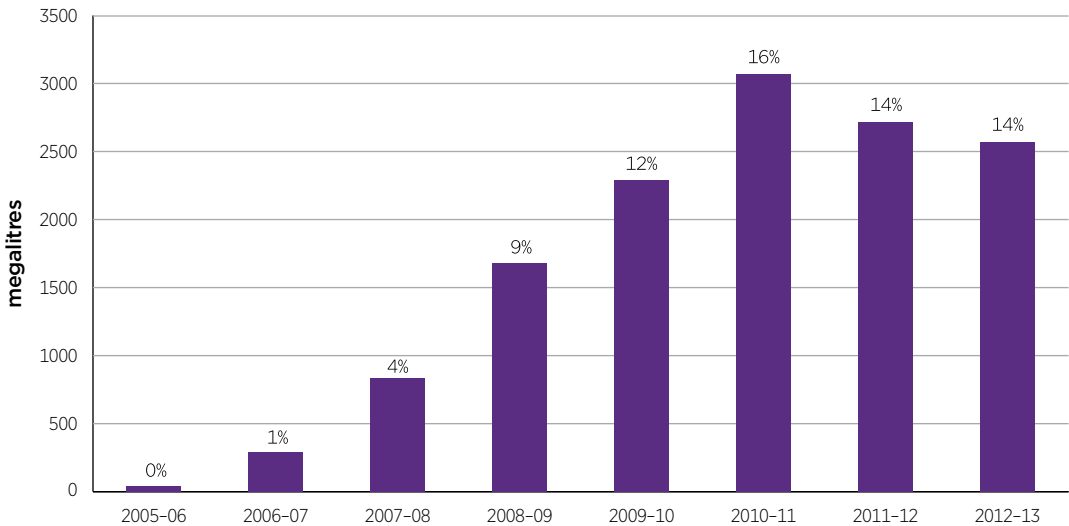
Chart 5.1 Total ethanol blended petrol sales by volume and as a proportion of total petrol sales: 2005–06 to 2012–13
